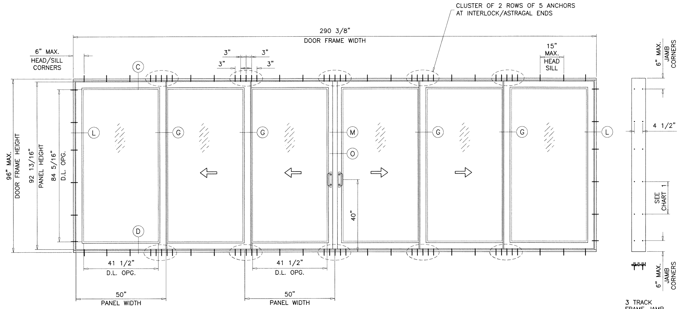
TYPICAL ELEVATION OXX-XXO
