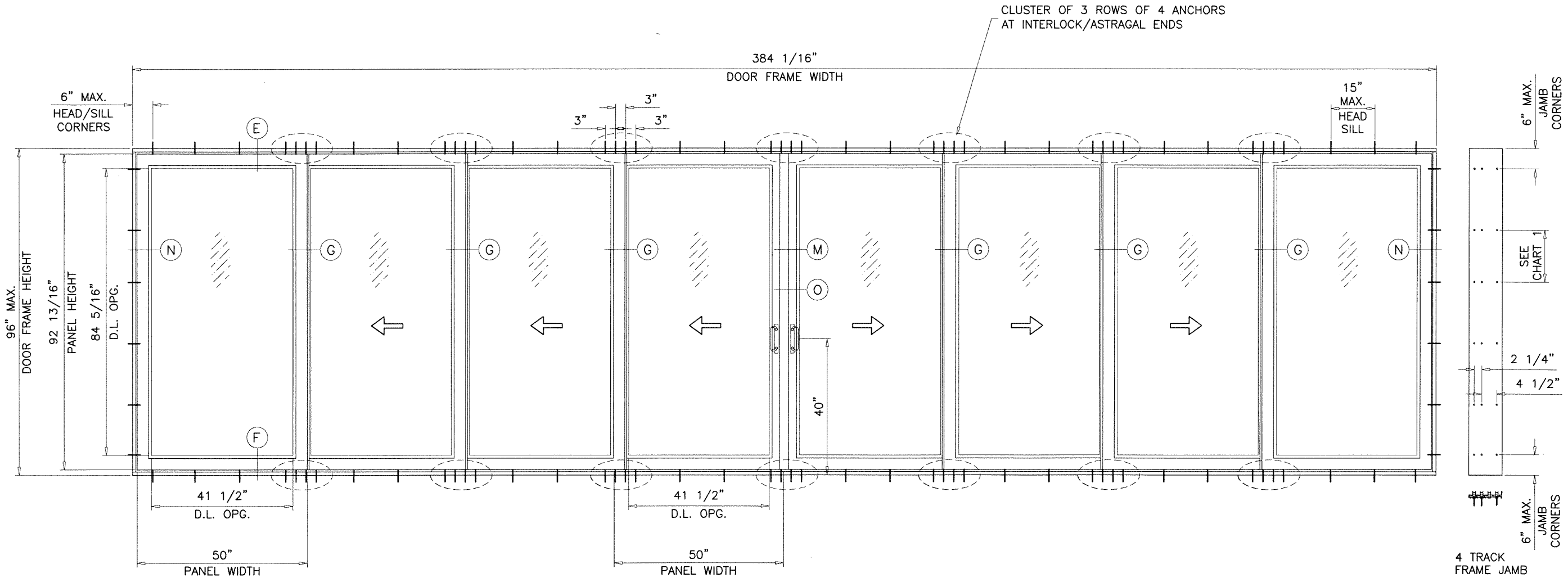
TYPICAL ELEVATION OXXX-XXXX
